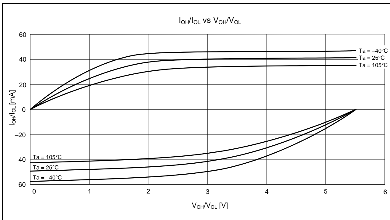
Figure 2.26 V_{OH}/V_{OL} and I_{OH}/I_{OL} Temperature Characteristics at V_{CC} = 5.5\text{ V} When Normal Drive Output is Selected (Reference Data)
