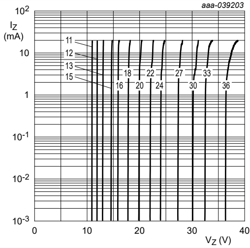
Fig. 7. Reverse current as a function of reverse voltage; typical values (BZX8450-B/C11 to BZX8450-B/C36)
