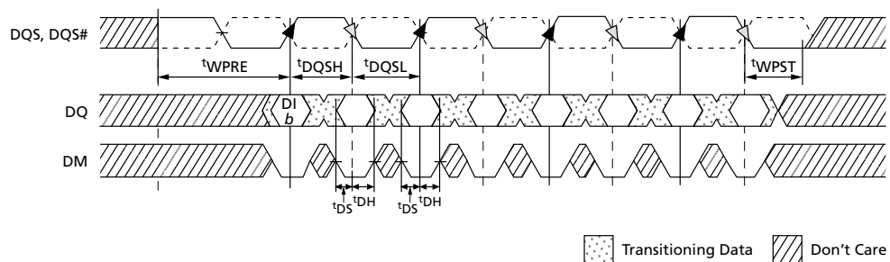
Figure 92: Data Input Timing
