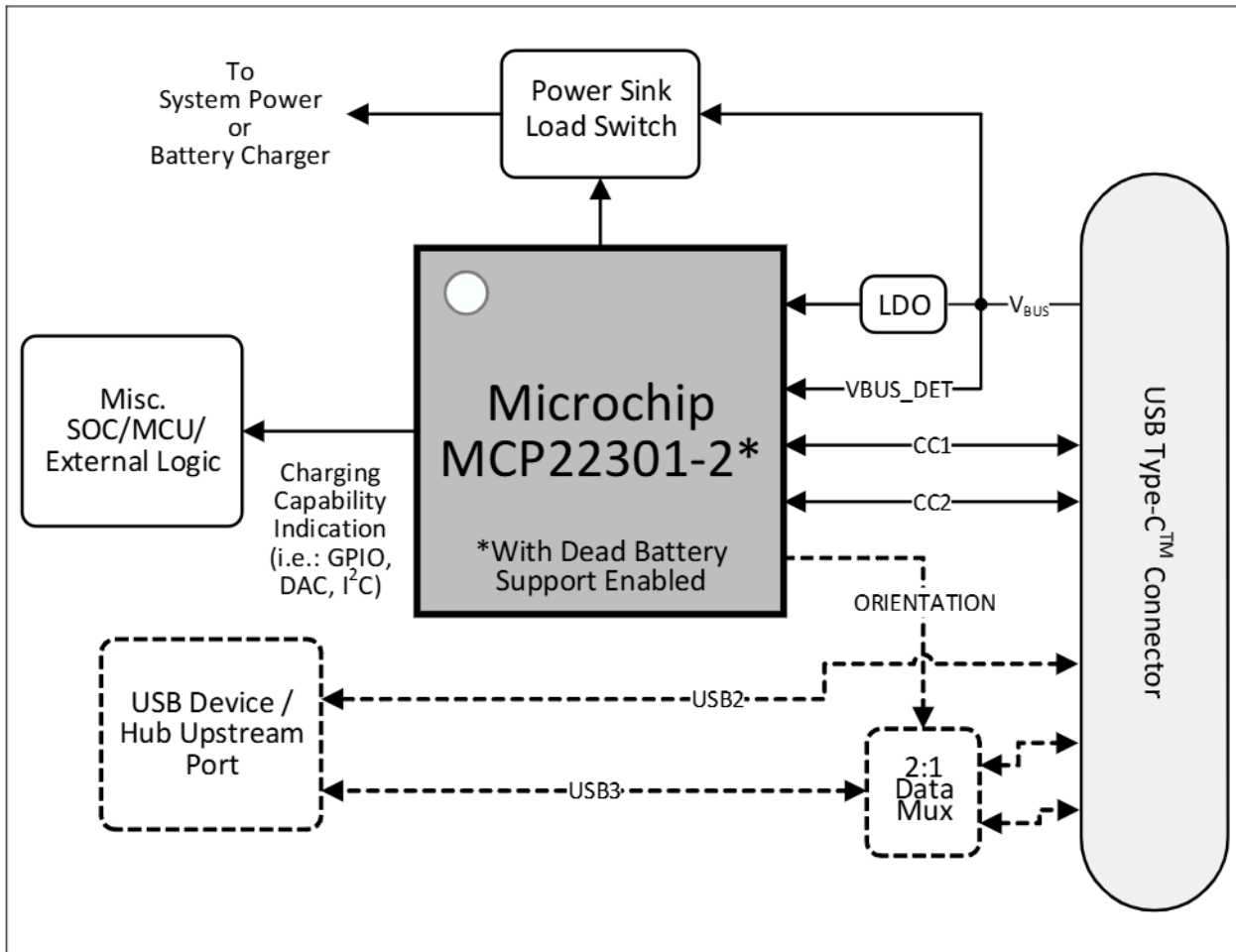
FIGURE 2-3: System Block Diagram - Sink-Only Application.
