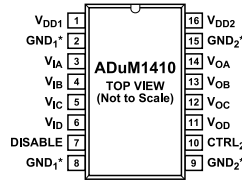
Figure 5. ADuM1410 Pin Configuration
