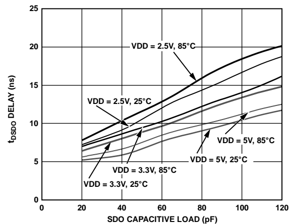
Figure 24. t_{pSDO} Delay vs. Capacitance Load and Supply
